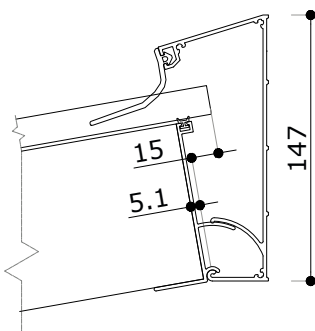
Wall profile Wandprofiel
